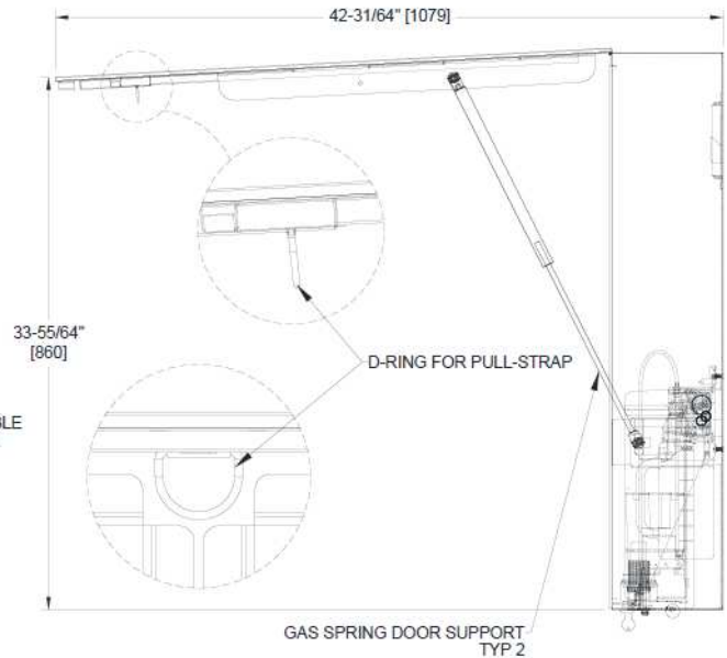
OPEN VIEW (-1, -2)
