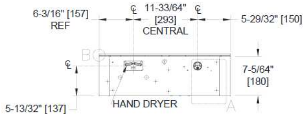
BOTTOM VIEW (-1, -2)
