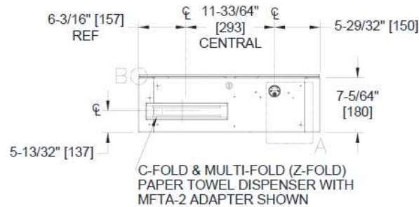
BOTTOM VIEW (-T)
