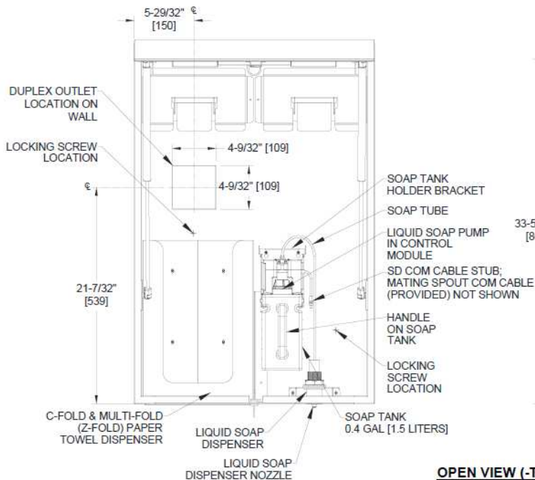
OPEN VIEW (-T)
